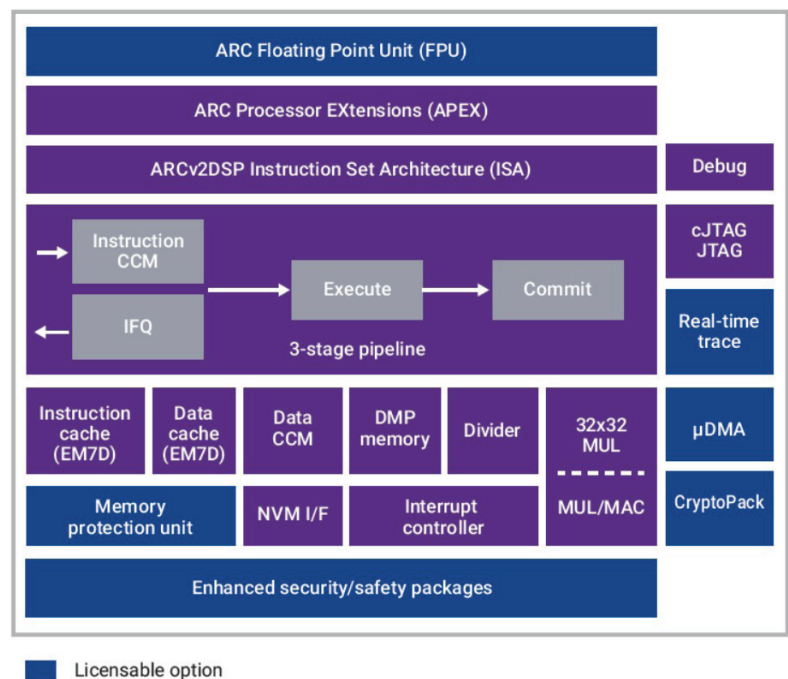
Figure 1: EM5D and EM7D Block Diagram
