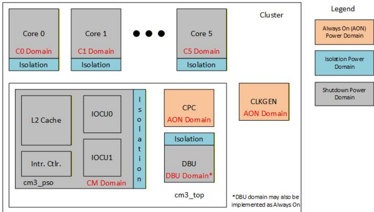
Figure 9.1 I8500 Power Domains
