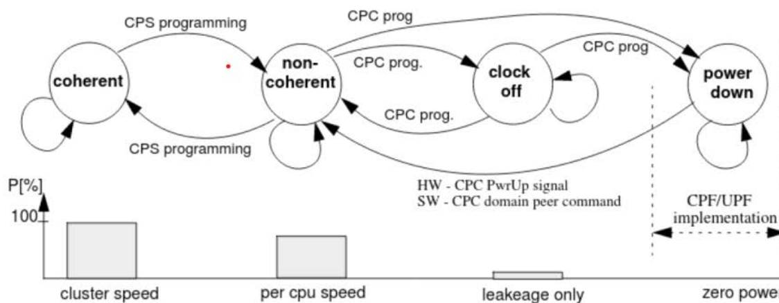
Figure 9.2 CPC Power State Transitions
