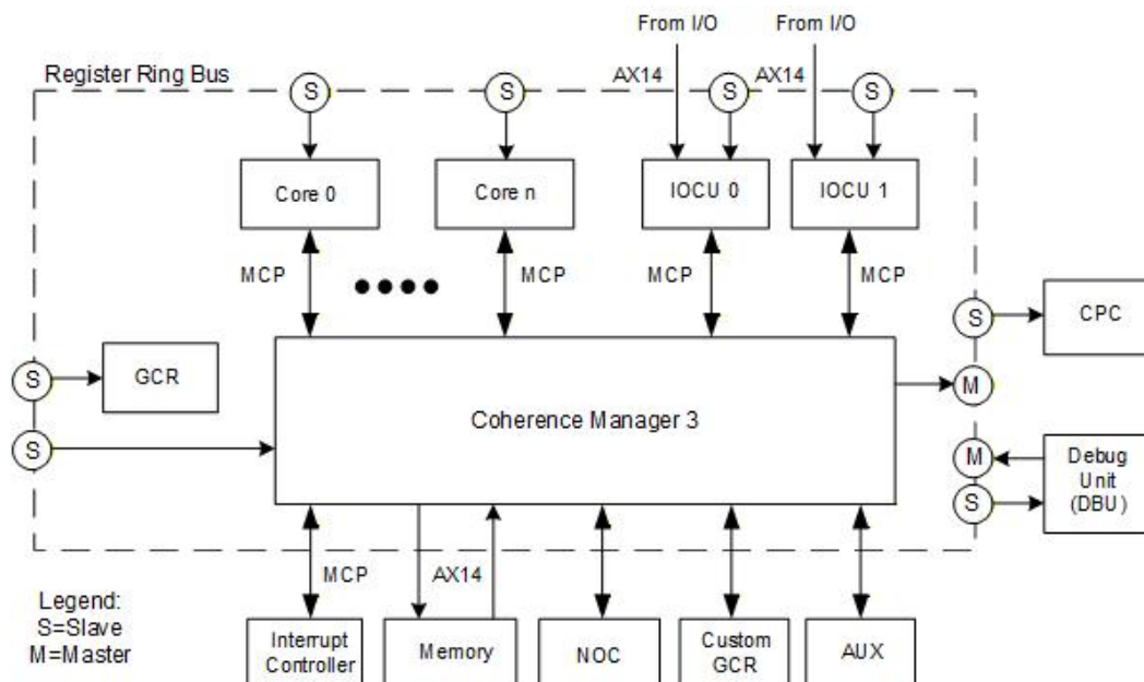
Figure 8.1 Interface Ports and Register Ring Bus Interface to the CM
