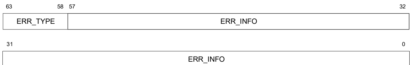
Figure 8.12 Global CM3 Error Cause Register Bit Assignments
