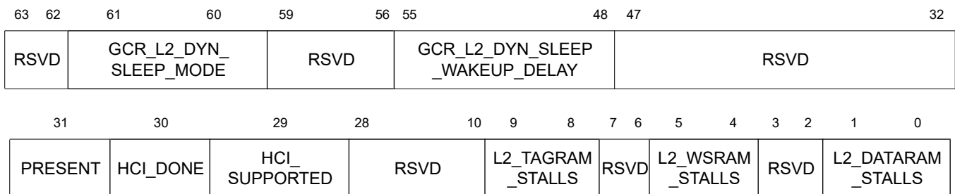
Figure 8.25 L2 RAM Configuration Register Bit Assignments
