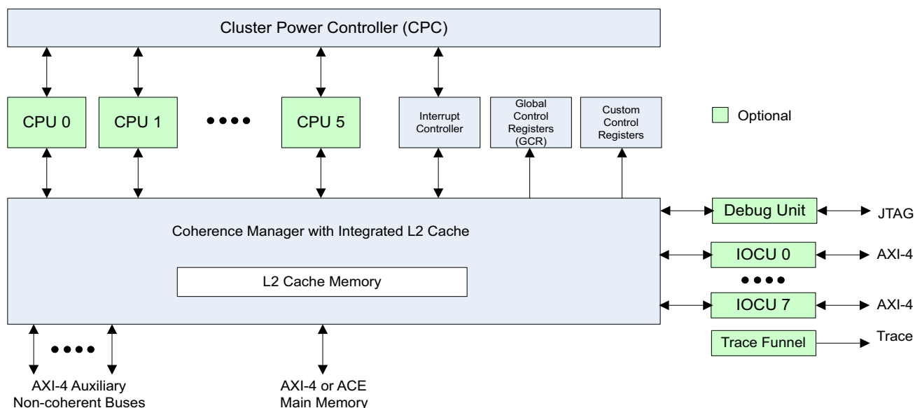
Figure 1.1 System-level Block Diagram of Single-Cluster MIPS Atlas I8500 Multiprocessing System
