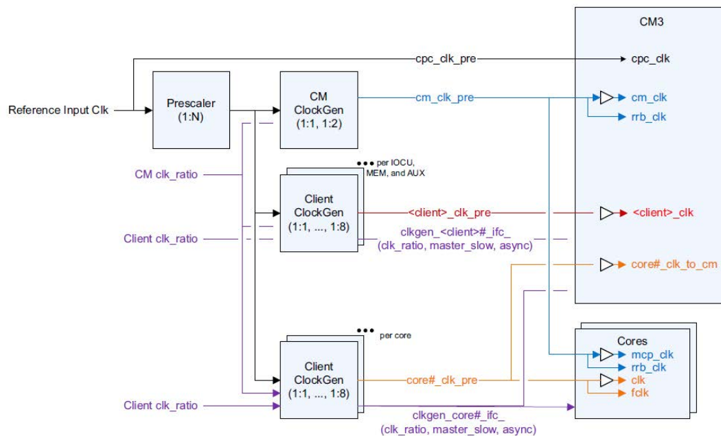
Figure 9.4 Top Level Clocking Diagram
