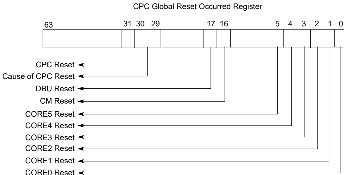
Figure 9.5 Reset Detection in the I8500 Multiprocessing System
