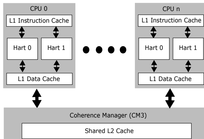
Figure 5.1 I8500 Multiprocessing System Caches
