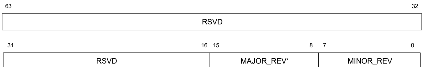
Figure 8.23 DBU Revision Register Bit Assignments
