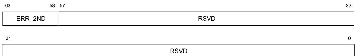
Figure 8.14 Global CM3 Error Multiple Register Bit Assignments
