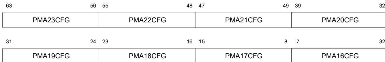
Figure 7.28 PMA Configuration 4 Control and Status Register Bit Assignments
