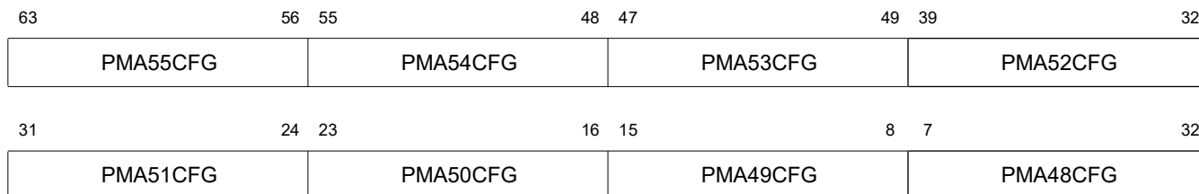
Figure 7.36 PMA Configuration 12 Control and Status Register Bit Assignments
