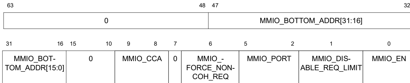
Figure 5.37 Global MMIO0 Bottom Register Bit Assignments
