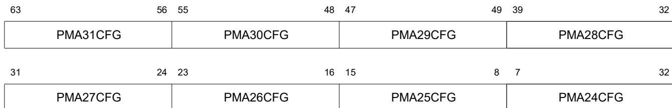
Figure 7.30 PMA Configuration 6 Control and Status Register Bit Assignments
