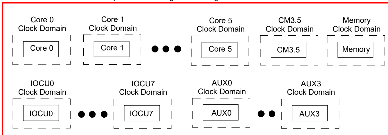
Figure 6.2 Clock Domains in the P8700-F Multiprocessing System
