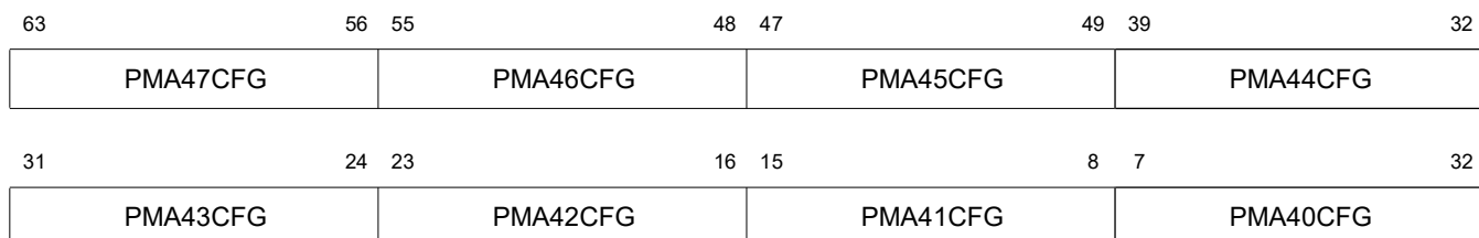
Figure 7.34 PMA Configuration 10 Control and Status Register Bit Assignments
