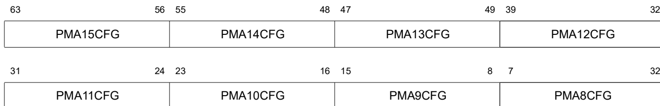
Figure 7.26 PMA Configuration 2 Control and Status Register Bit Assignments
