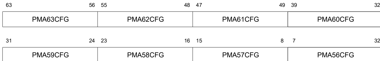
Figure 7.38 PMA Configuration 14 Control and Status Register Bit Assignments
