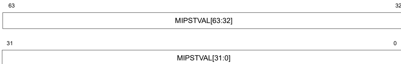
Figure 7.10 MIPS Trap Value Register Bit Assignments — RV64
