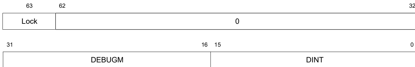
Figure 5.89 Power Debug Interrupt Register Bit Assignments
