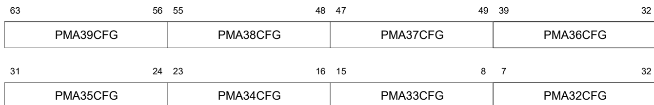
Figure 7.32 PMA Configuration 8 Control and Status Register Bit Assignments
