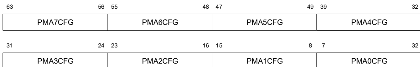
Figure 7.24 PMA Configuration 0 Control and Status Register Bit Assignments
