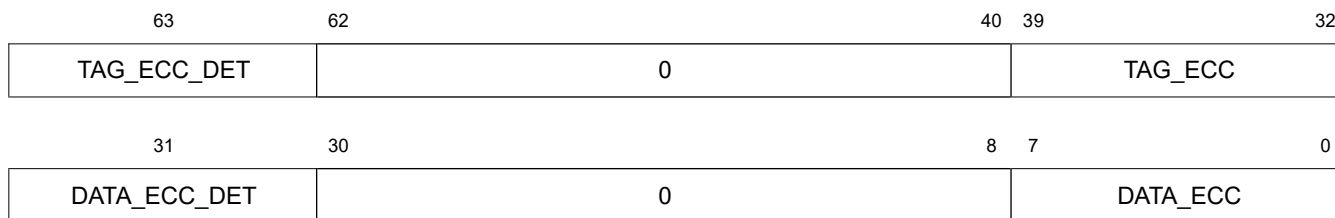
Figure 5.31 Global L2 ECC Register Bit Assignments
