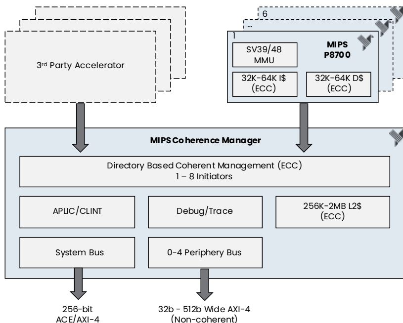
Figure 2: MIPS™ P8700 Multi-Processing System
