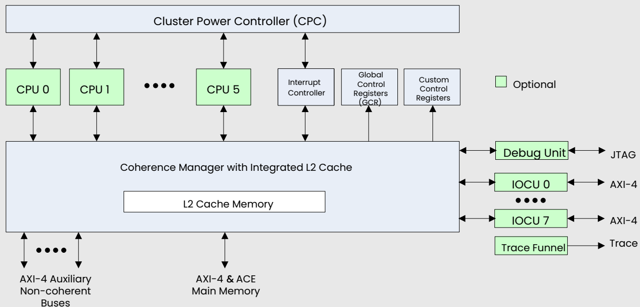
Figure 1. P8700 Multiprocessing System Block Diagram
