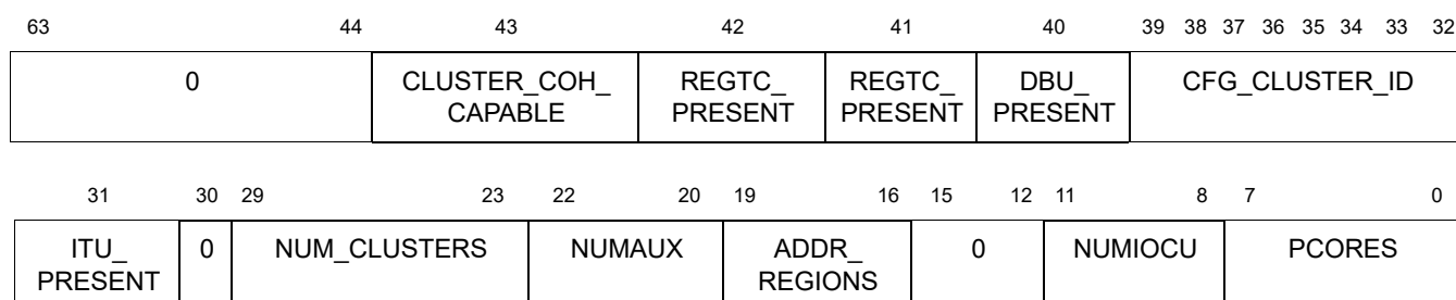
Figure 5.4 GCR Global Configuration Register Bit Assignments
