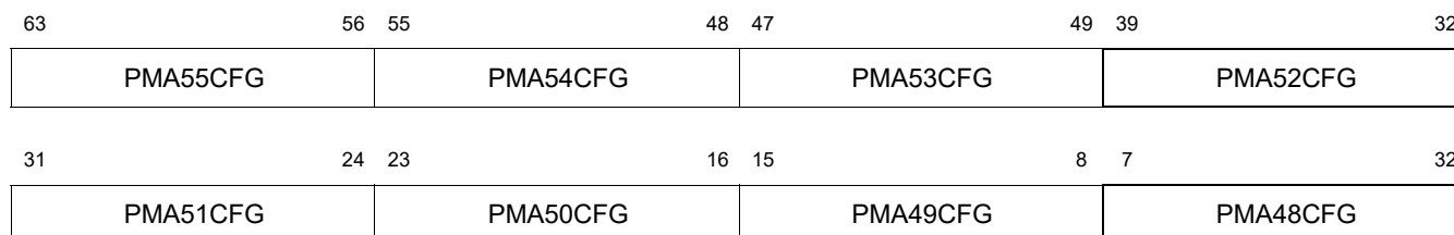
Figure 7.38 PMA Configuration 12 Control and Status Register Bit Assignments
