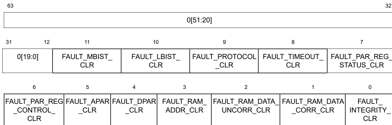
Figure 5.93 Power Fault Clear Register Bit Assignments
