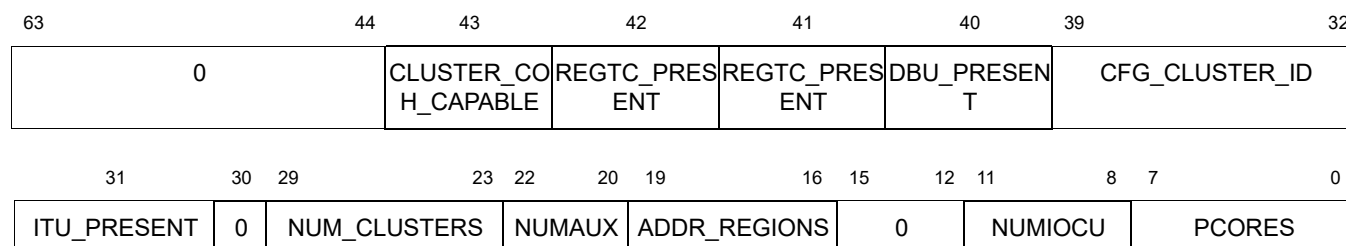
Figure 5.82 Global Configuration Register Bit Assignments
