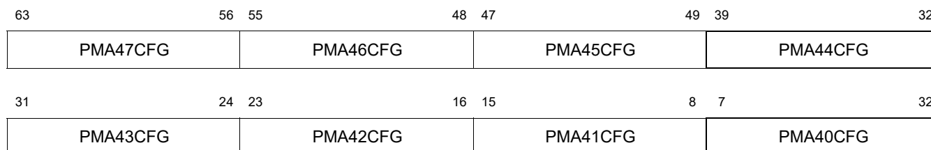
Figure 7.36 PMA Configuration 10 Control and Status Register Bit Assignments
