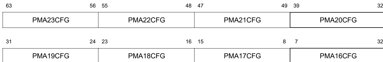
Figure 7.30 PMA Configuration 4 Control and Status Register Bit Assignments
