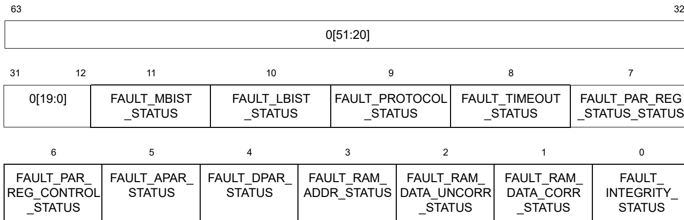
Figure 5.78 Global Fault Status Register Bit Assignments
