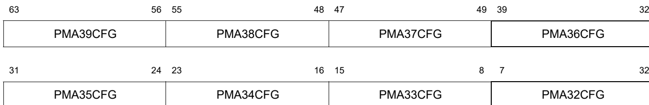
Figure 7.34 PMA Configuration 8 Control and Status Register Bit Assignments
