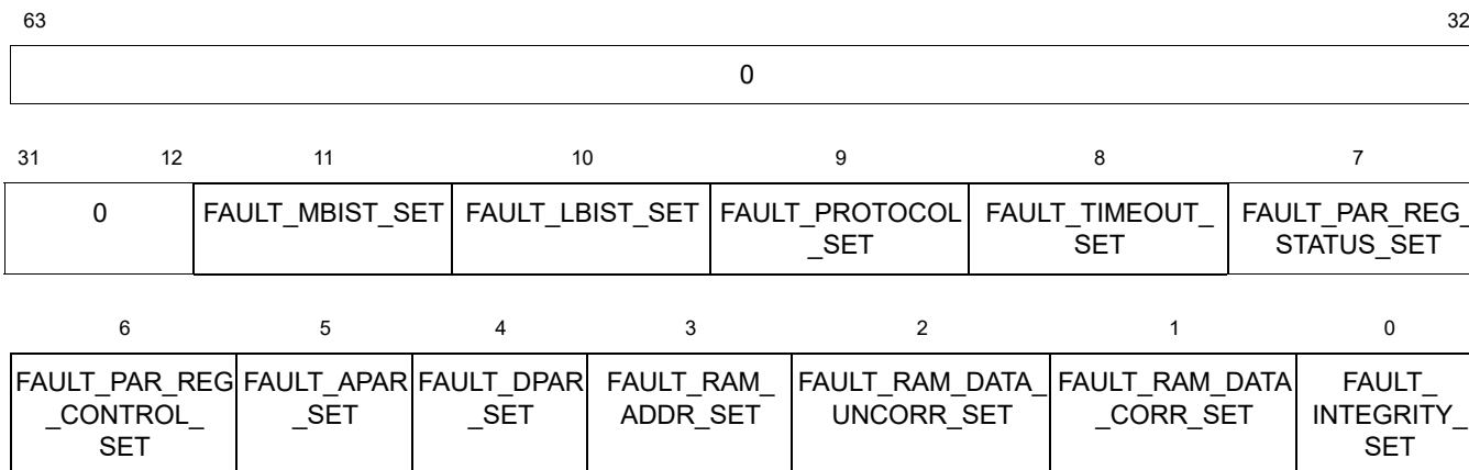
Figure 5.92 Power Fault Set Register Bit Assignments
